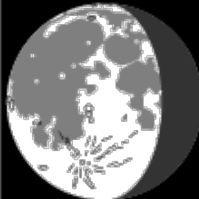
gibbous waning
