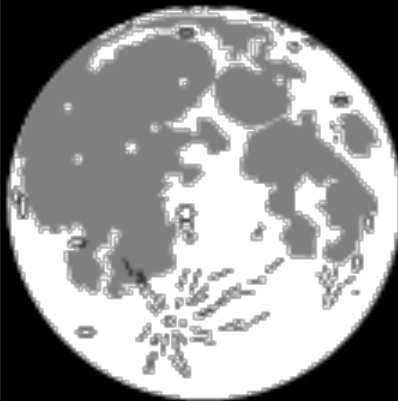
full
