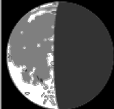
half-moon waning
