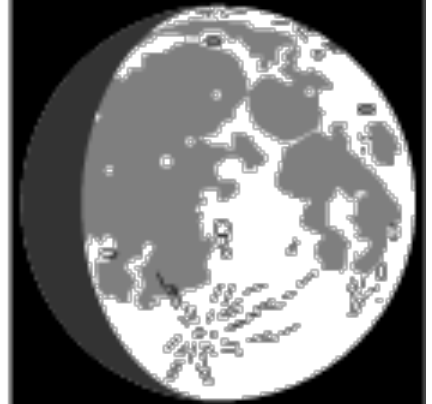
gibbous waxing
