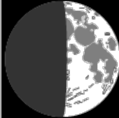
half-moon waxing
